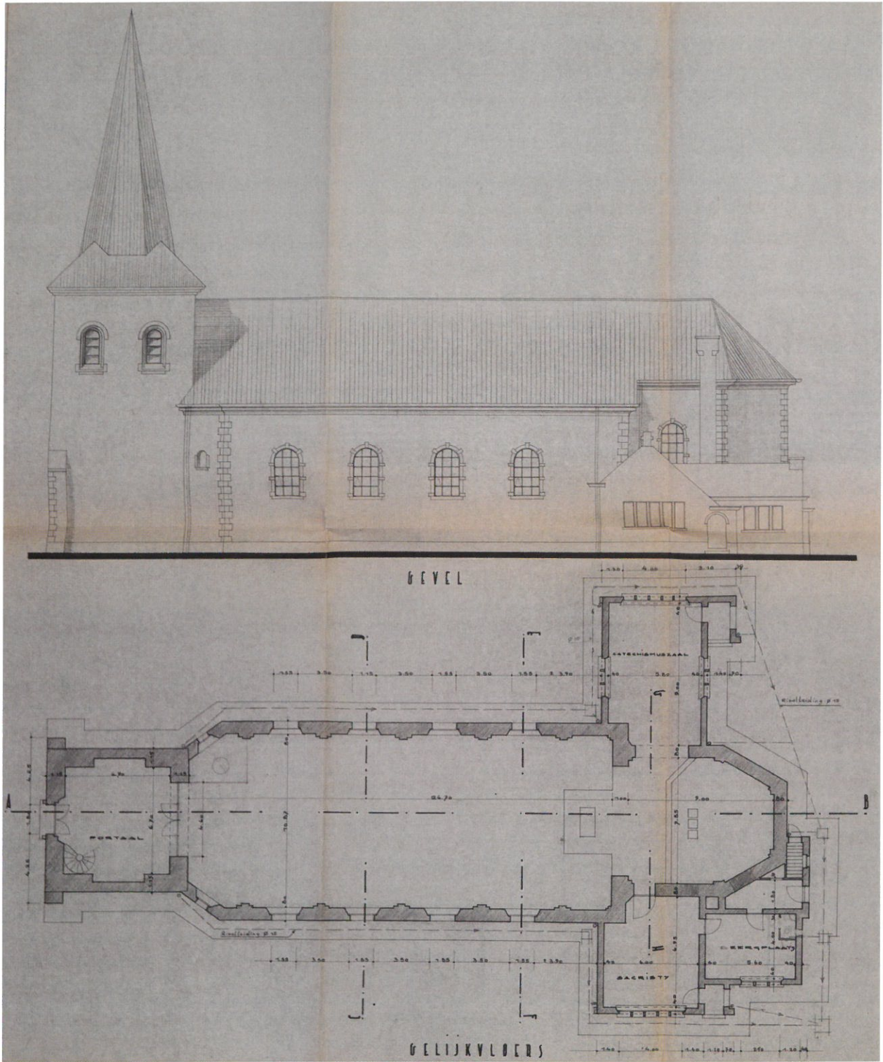
Plannen van architect Gessler
